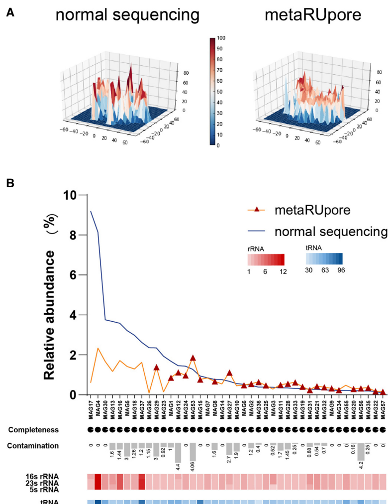
Figure 3. Performance of metaRUpore on recovery of high-quality MAGs in TAD community. (A) 3D density plots of t-SNE downscaling results for normal sequencing data sets and selective sequencing data sets by metaRUpore at four base frequencies, showing that metaRUpore renders the TAD community structure homogenous. (B) The distribution of 41 retrieved HQ MAGs in normal and RU sequencing data set. The red triangles indicate MAGs that could only be assembled in the metaRUpore data set. The pie chart and bar chart represent the level of genomic SCG-completeness and contamination by CheckM. The copy numbers of 16S rRNA, 23S rRNA, and 5S rRNA ribosomal RNA genes are represented by the red heatmap, whereas the copy number of tRNA is represented by the blue heatmap.
