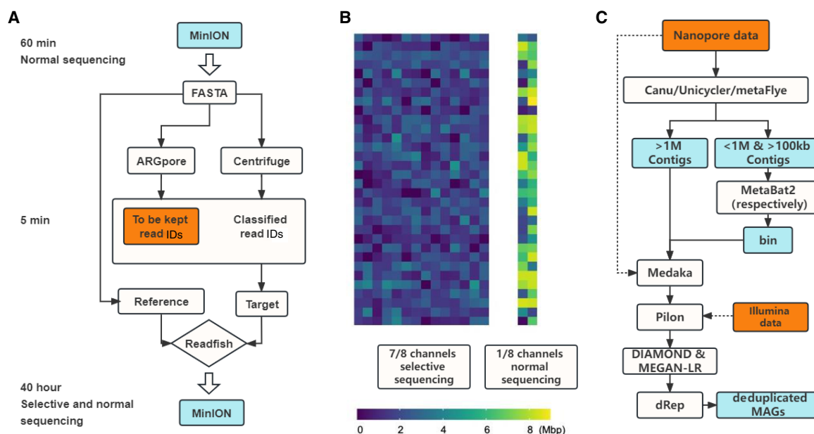
Figure 2. The workflow of metaRUpore and bioinformatic analysis. (A) The workflow of metaRUpore. (B) A MinION flow cell in metaRUpore is configured into two parts, 1/8th of the channels for normal sequencing and the remaining channels for selective sequencing. (C) The bioinformatic workflow for HQ-MAGs retrieval based on data sets derived from nanopore selective sequencing and Illumina sequencing.
